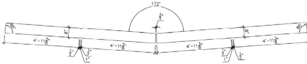
PLAN
